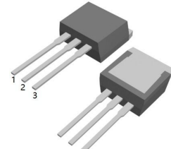
TO-262-3L HBR10100HCT
