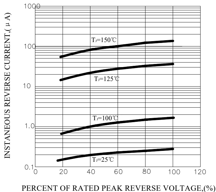
FIG.5-TYPICAL REVERSE CHARACTERISTICS
