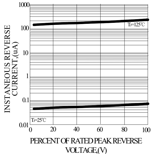
FIG.4-TYPICAL REVERSE CHARACTERISTICS
