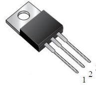
TO-220AB-3L MBR40100CT
