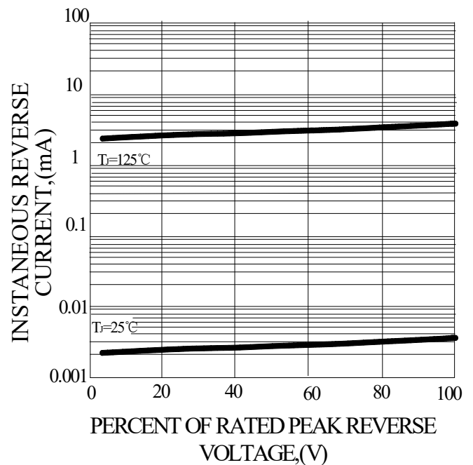
FIG.4-TYPICAL REVERSE CHARACTERISTICS
