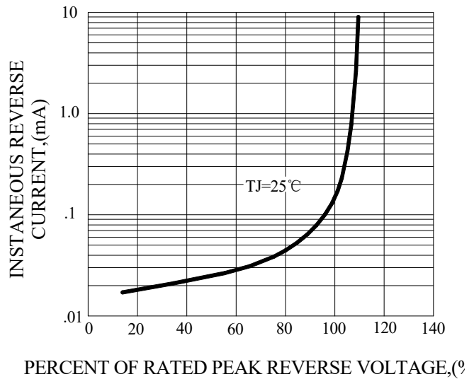
FIG.4-TYPICAL REVERSE CHARACTERISTICS
