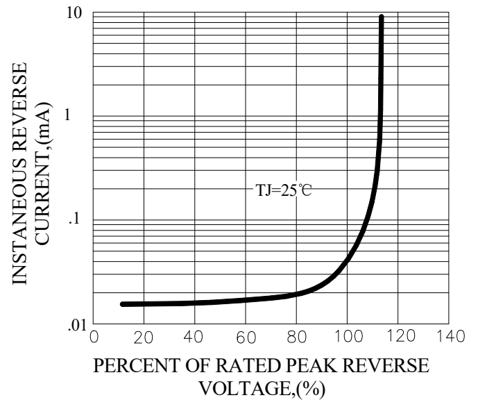
FIG.4-TYPICAL REVERSE CHARACTERISTICS
