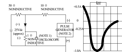
FIG.5-TEST CIRCUIT DIAGRAM AND REVERSE RECOVERY TIME CHARACTERISTIC
