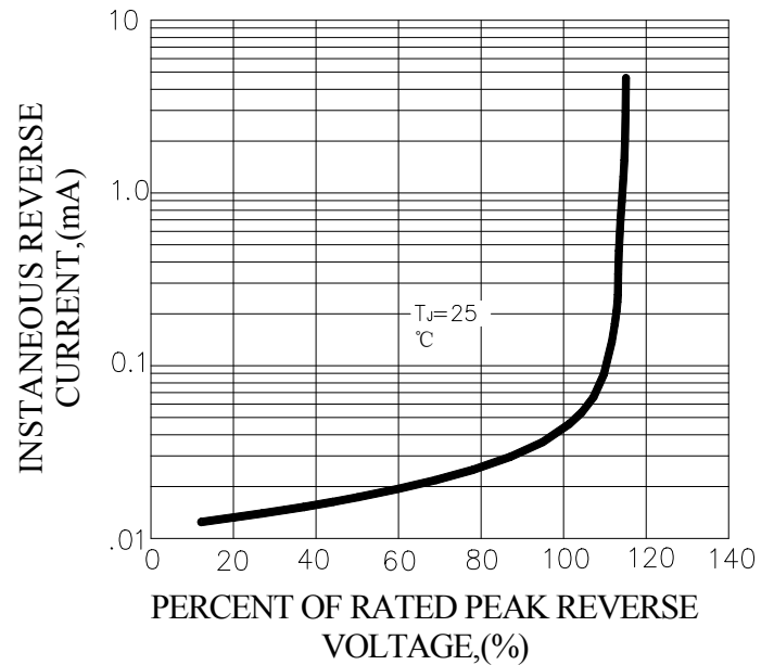
FIG.4-TYPICAL REVERSE CHARACTERISTICS
