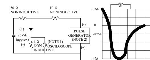
FIG.5-TEST CIRCUIT DIAGRAM AND REVERSE RECOVERY TIME CHARACTERISTIC
